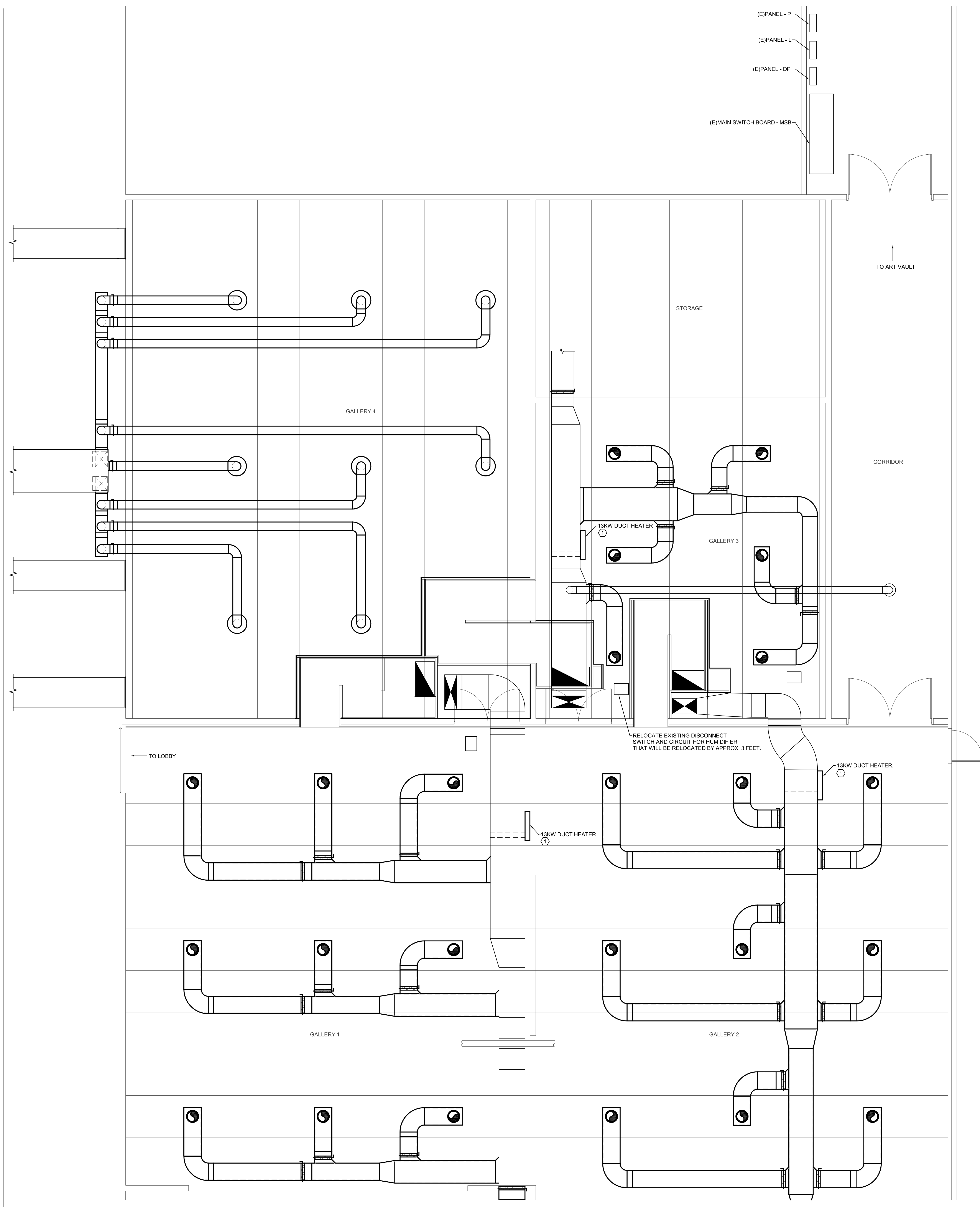
1 ELECTRICAL FLOOR PLAN SCALE: 1/4" = 1'-0"
